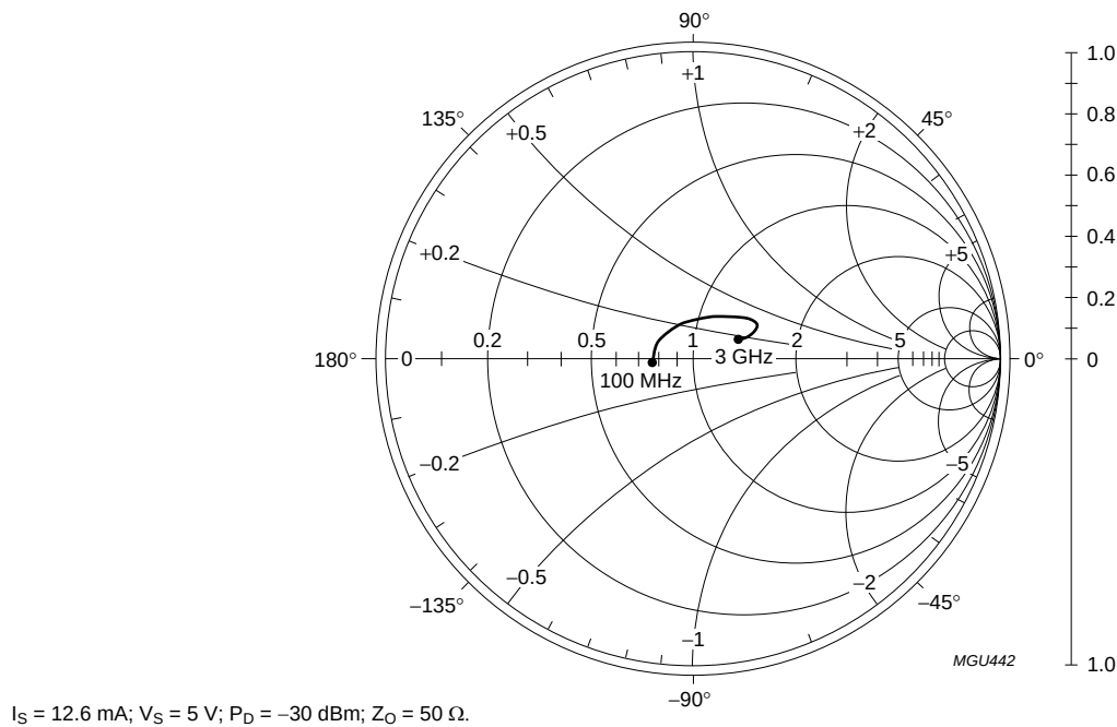
Fig.8 Output reflection coefficient ( s_{22} ); typical values.
