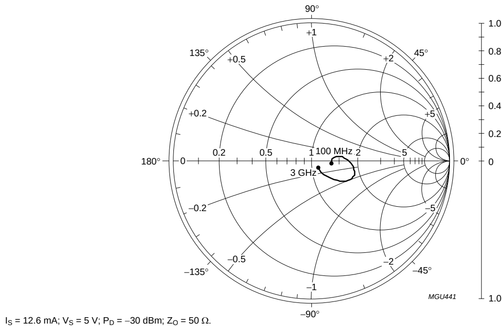
Fig.7 Input reflection coefficient ( s_{11} ); typical values.
